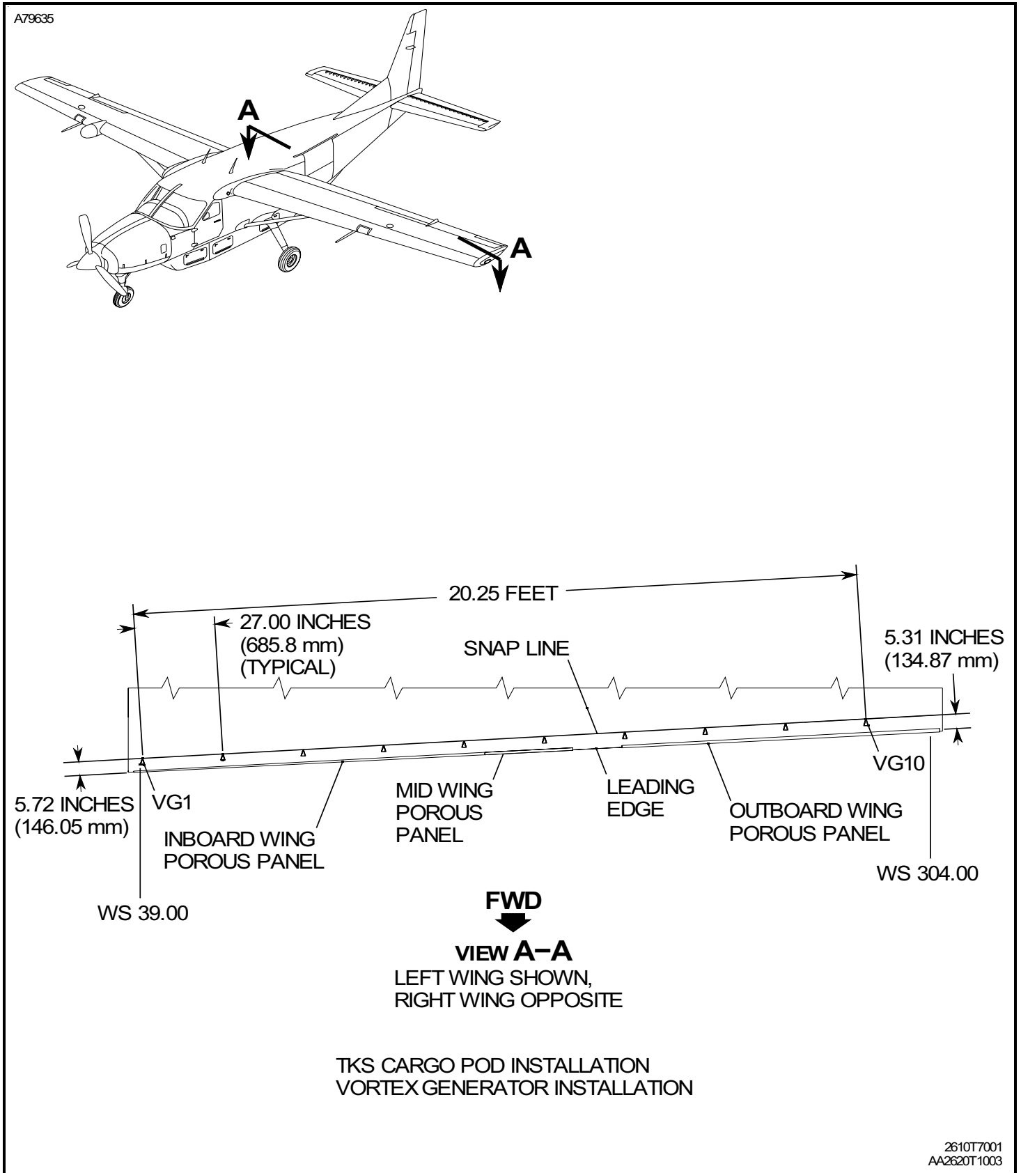
Figure 201 : Sheet 1 : TKS Cargo Pod Vortex Generator Installation
