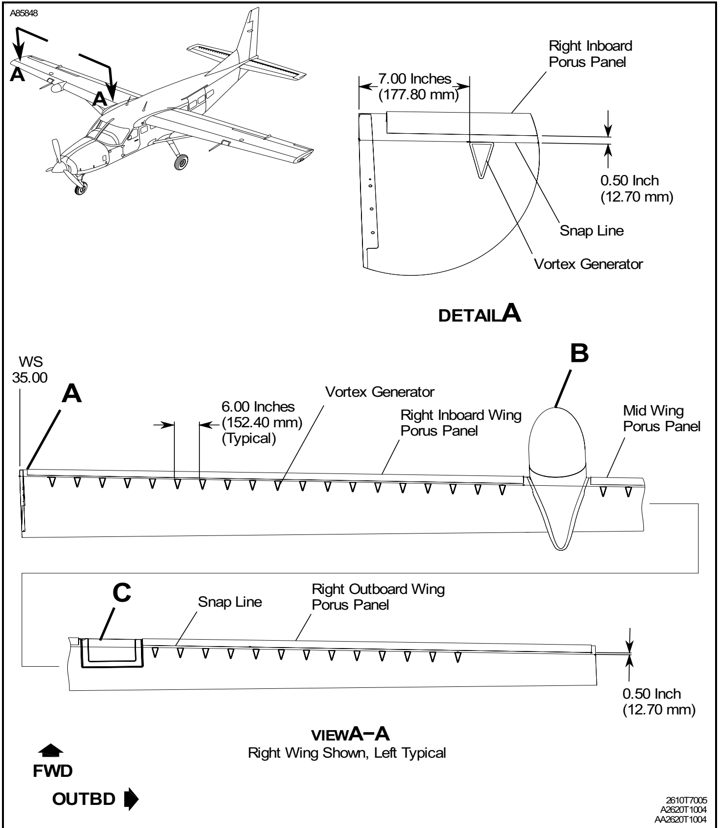
Figure 202 : Sheet 1 : TKS Fairing Vortex Generator Installation
